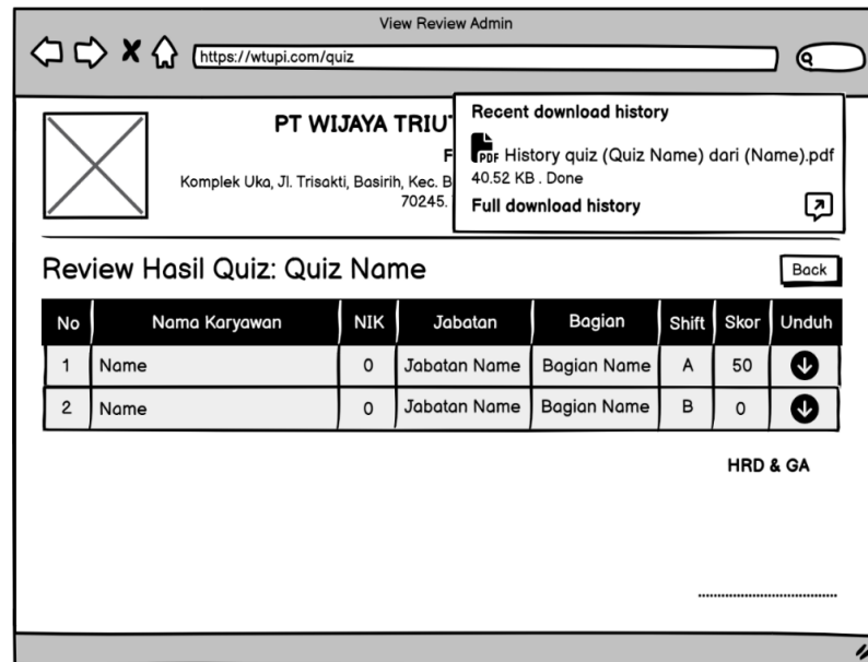
Gambar 3.36 Mockup Tombol Unduh View, Menu Review Admin
