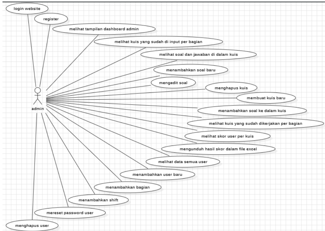
Gambar 3.14 Use Case Diagram Admin
