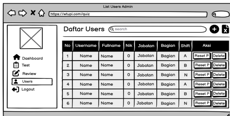
Gambar 3.39 Mockup Halaman Users Admin
