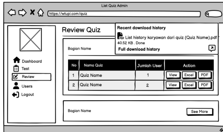
Gambar 3.38 Mockup Tombol Export PDF , Menu Review Admin
