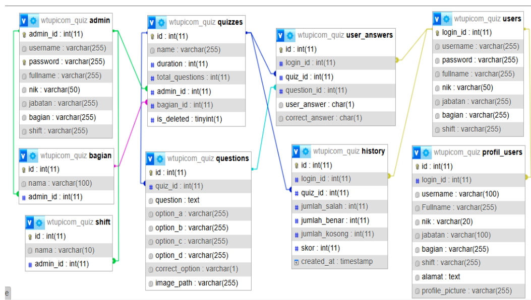
Gambar 3.16 Relasi Tabel Database
