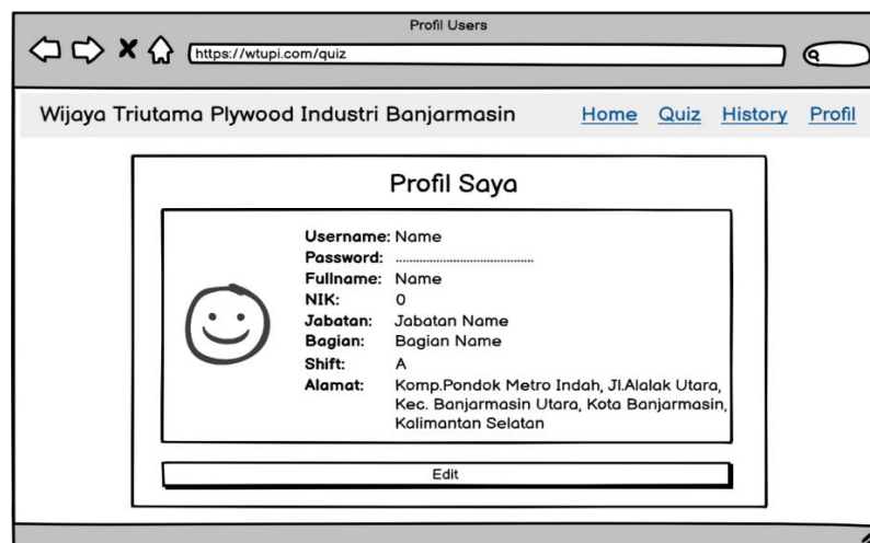
Gambar 3.52 Mockup Halaman Profil User
